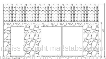
FACHADA PRINCIPAL
