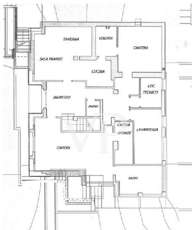
PIANO SEMINTERRATO
