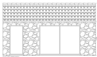
FACHADA PRINCIPAL
